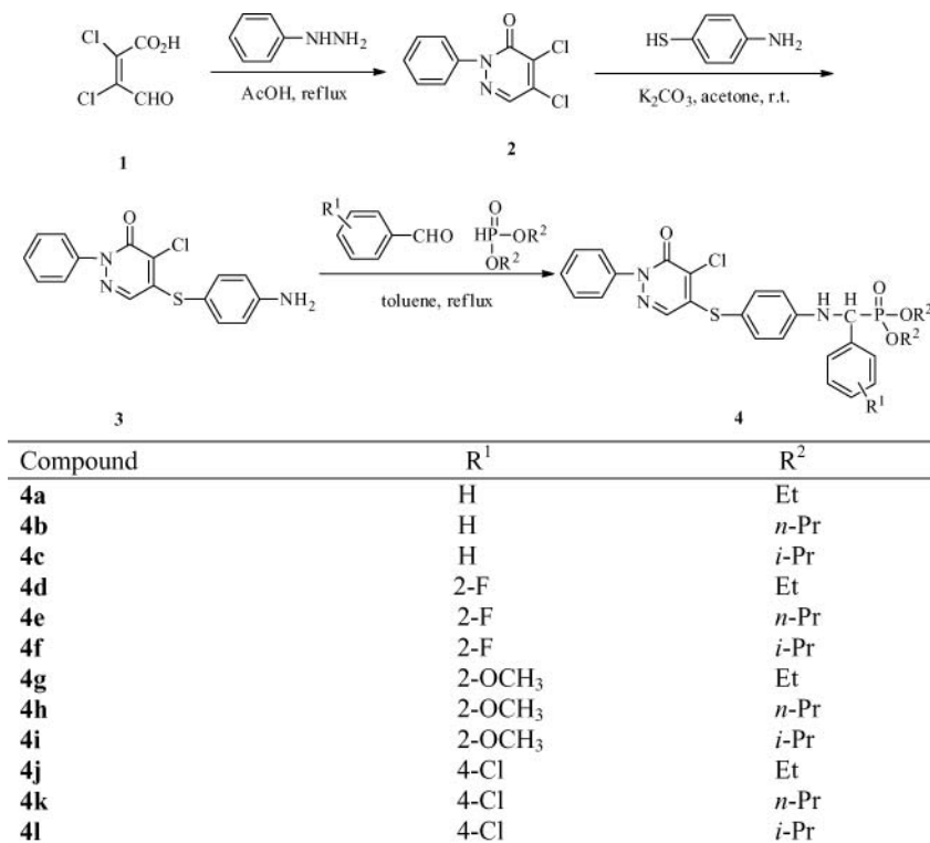
Scheme 1 Synthetic route to title compounds 4.
